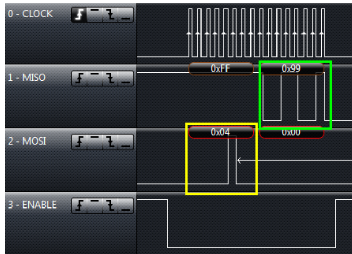
Figure 4-7. Waveform Graph 3
